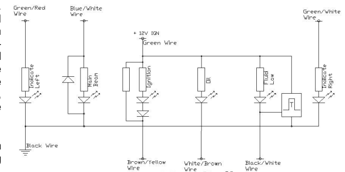
Figure 3. Circuit diagram
