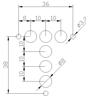
Figure 2. Drill dimensions
