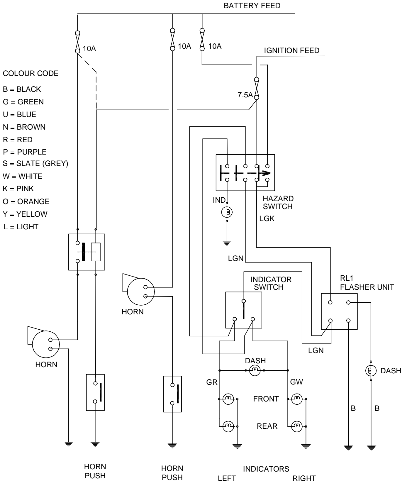
CIRCUIT DIAGRAM FOR HORN, HAZARDS & INDICATORS
