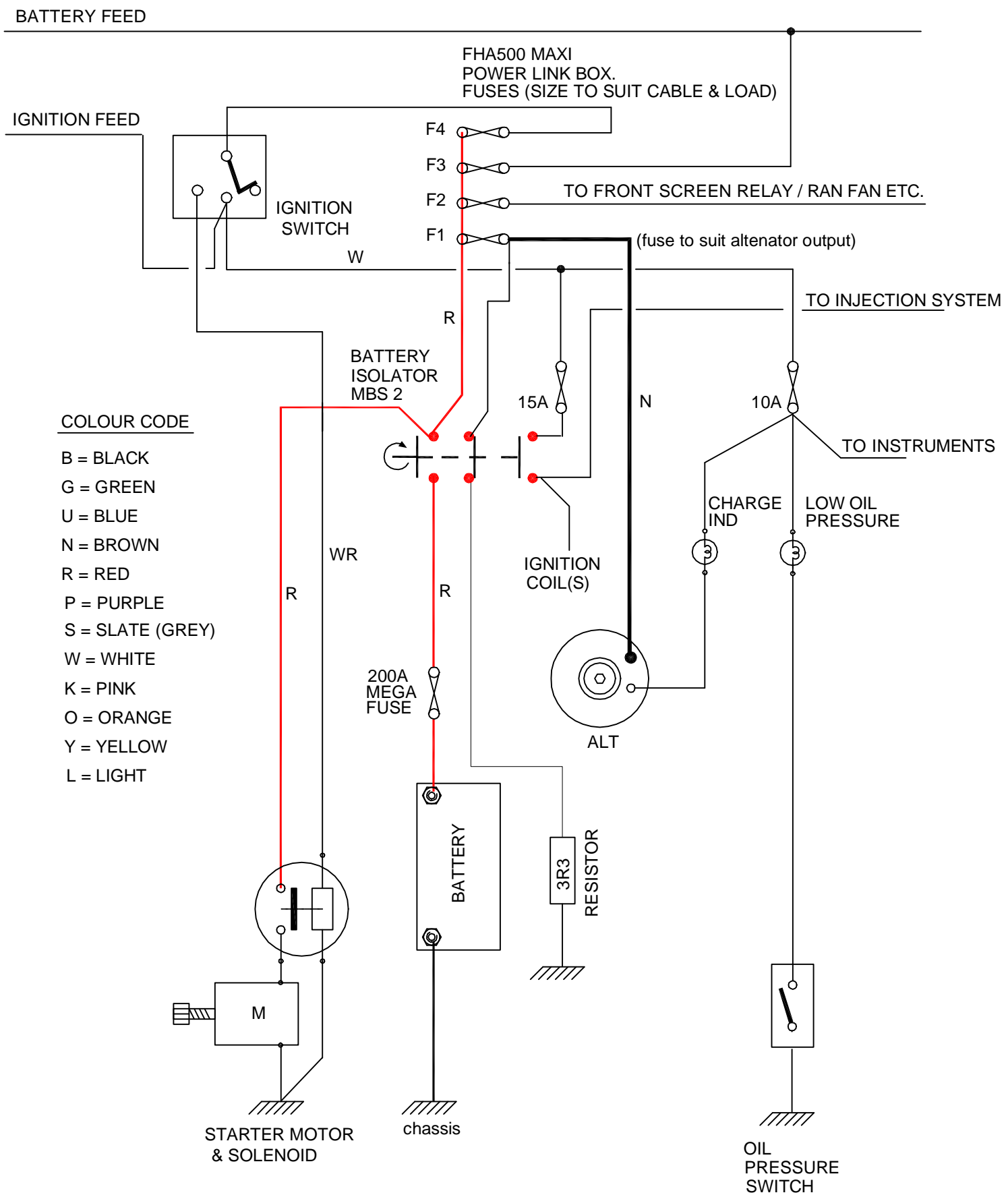
CIRCUIT DIAGRAM FOR START & CHARGE SECTION
